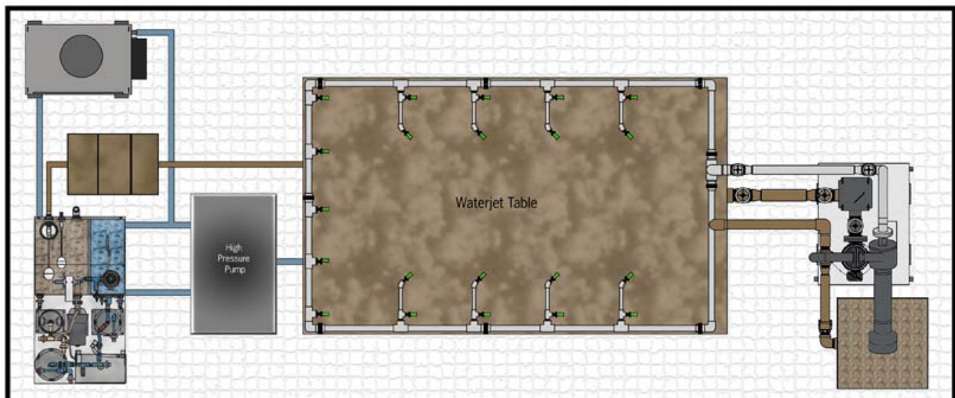
Closed Loop with Settling Weir & Chiller Typical Layout Abrasive Removal also shown
